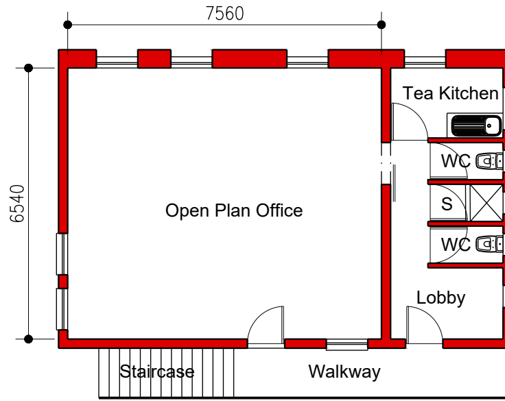
First Floor Layout
