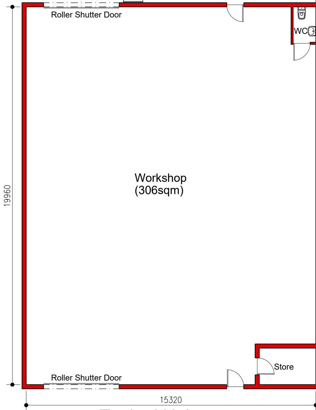
Typical Unit Ground Floor Layout
